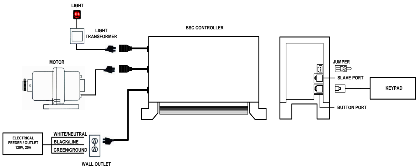
Fig. 1 Wiring Connection Diagram
