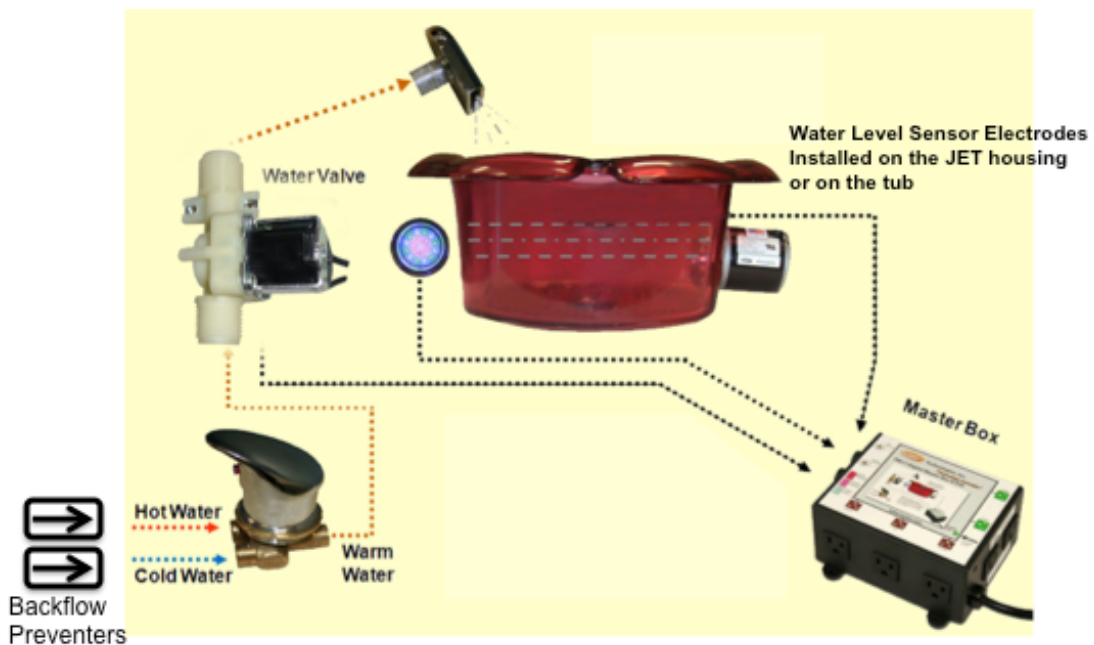
Fig.1: Connection Diagram
